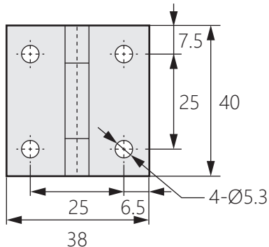
[OH-0337-2] 鍍鎳
