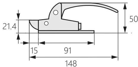
〔TH-52-1扣座〕
