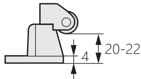
〔TH-52-2扣座〕
